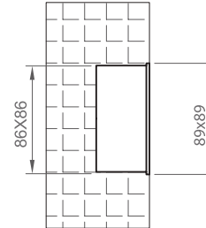
Concrete Wall
