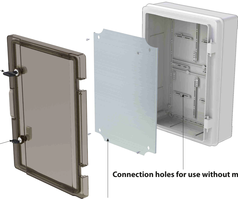
Galvanized sheet metal mounting plate
