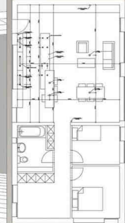
PLAN PLAFON Sc. 1/50
