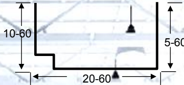
CRACKED CORNER U PROFILE
