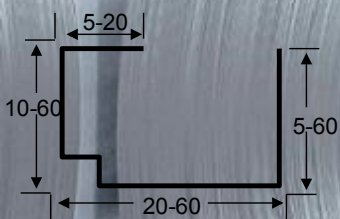
CRACKED CORNER G PROFILE
