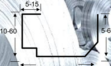
CRACKED CORNER ANGELED G PROFILE
