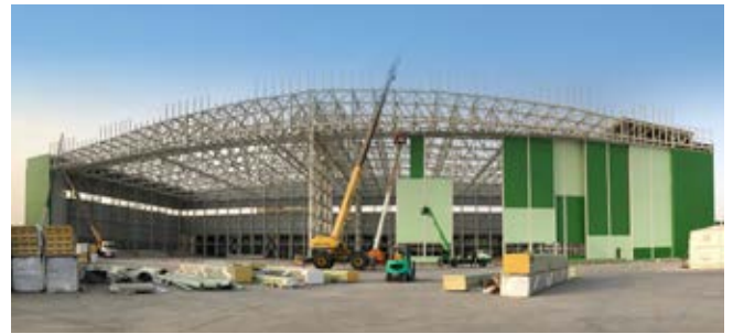
AIRCRAFT MAINTENANCE HANGAR FOR IRAQI AIRWAYS BAGHDAD / IRAQ
