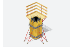
H20/P Plywood Faced Column Form System
