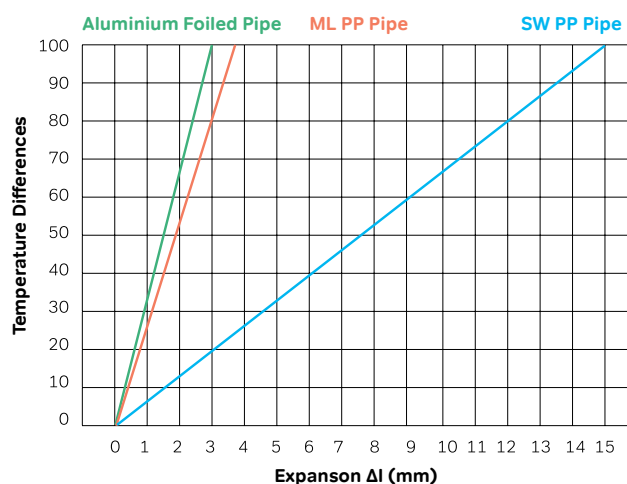
Graphic 1: Elongation of various PP pipes
