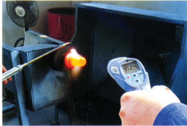
Temperature control of a plunger during fusion
