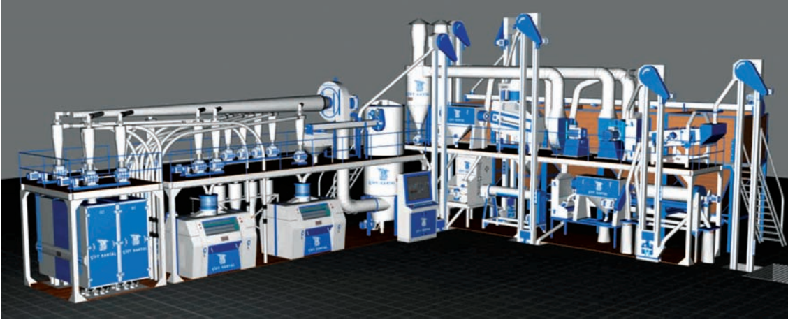
2 VALSLİ KOMPAKT TESİSİ COMPACT FLOUR MILL PLANT WITH 2 ROLLER MILL
