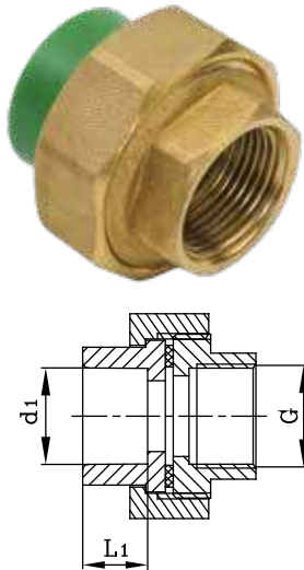
Metal Female Threaded Union (Hexagonal Shaped)
