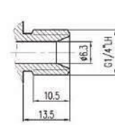
EN16129-H.4-G1/4"LH
