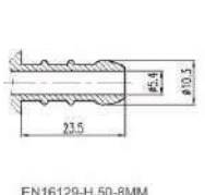
EN16129-H.50-8MM
