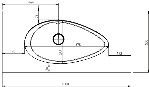
Bathroom Sink Dimensions
