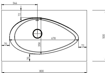
Bathroom Sink Dimensions
