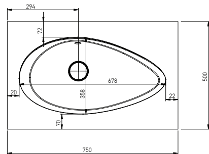
Bathroom Sink Dimensions
