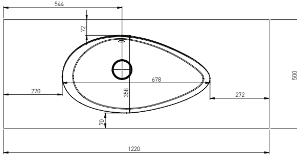
Bathroom Sink Dimensions
