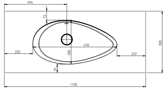
Bathroom Sink Dimensions
